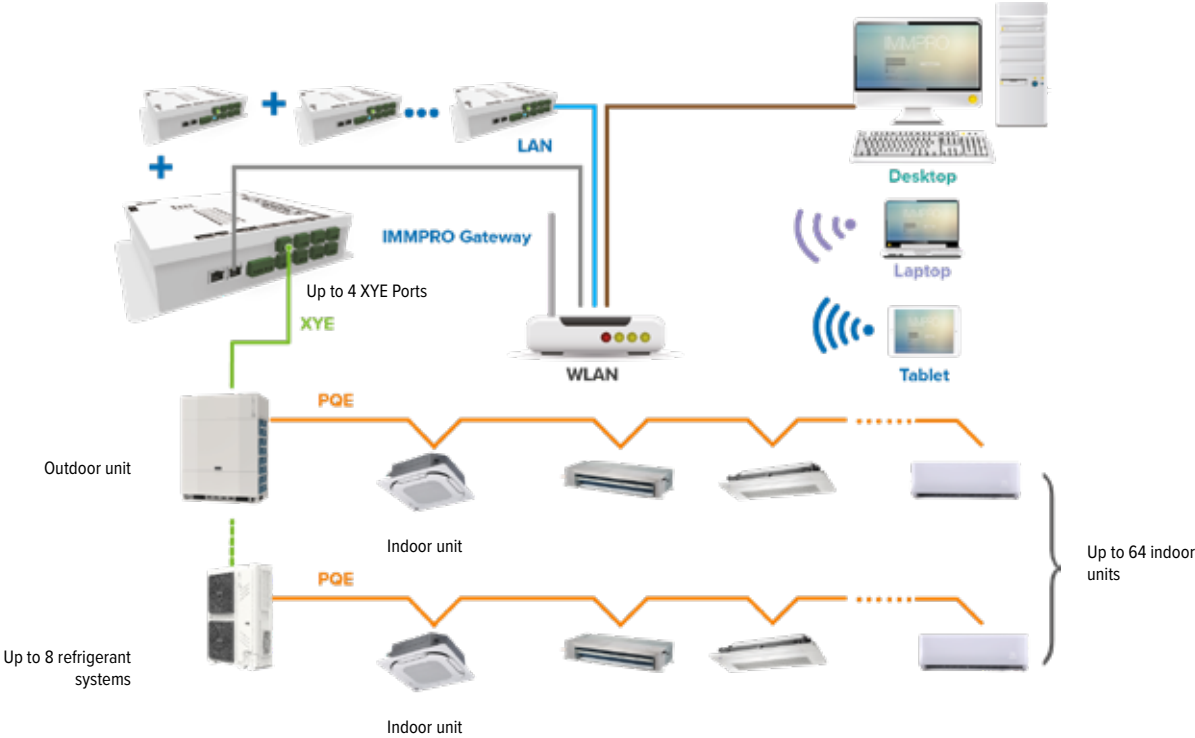
Wiring diagram with IMMPRO-BAC or IMMPRO-BAC(A) as IMMPRO gateway
